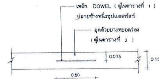
CONTRACTION JOINT
