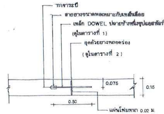
EXPANSION JOINT
